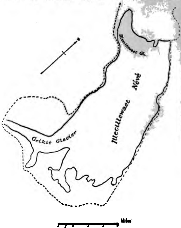
FIG. 415. — Outline map of the Illecillewaet glacier, an inherited-basin glacier in the Selkirks.
